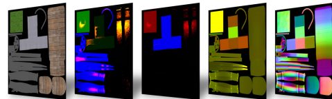
Figure 4: The material atlas contains all surface information. In this image a subset of the atlas textures is shown. From left to right: original colors, amount of the respective material types (two images), texel-to-world scale and surface normals.
